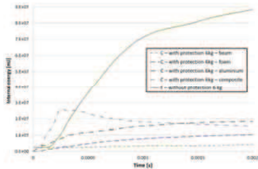
Fig. 8. Internal energy of the pillar and panel components
