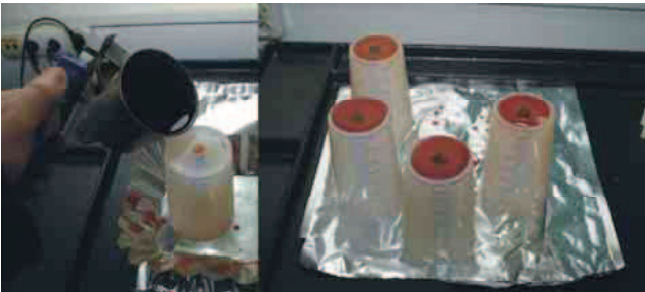
Fig. 5. Silicone mould pouring cylinder core wax model
