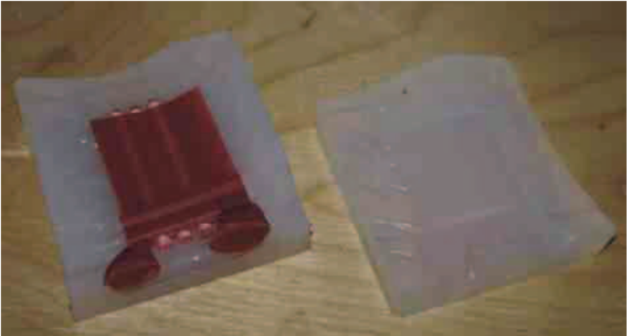
Fig. 4. Wax model of core blade and silicone mould
