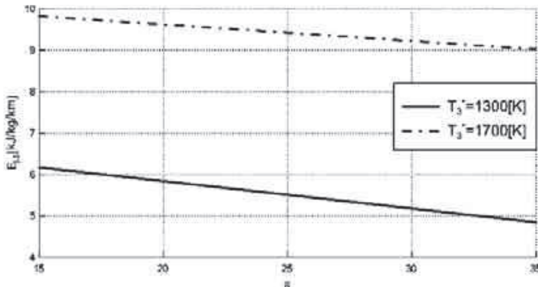
Fig. 8. Influence of the change of the compressor's compression \pi_{\Sigma}^* and temperature T_3^* on the unitary energy consumption E_{j,\Sigma}
