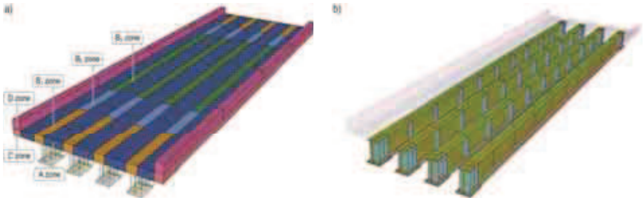
Fig. 6. The FE model of the KNI 140070 viaduct superstructure – FE parts and homogenization zones are marked
