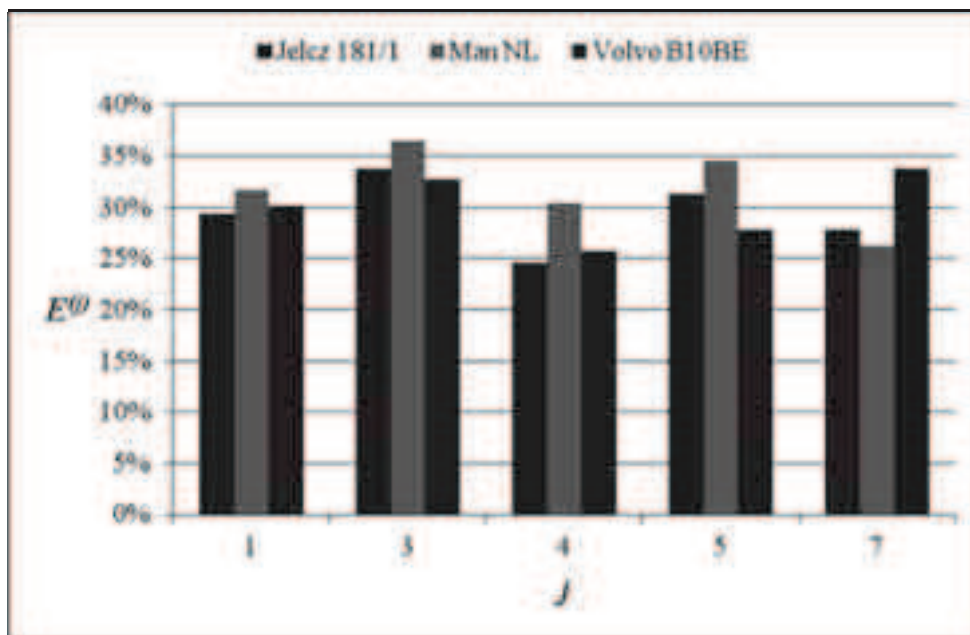
Fig. 1. The values of repair efficiency index performed in the emergency repair subsystem, determined for selected systems of urban buses
