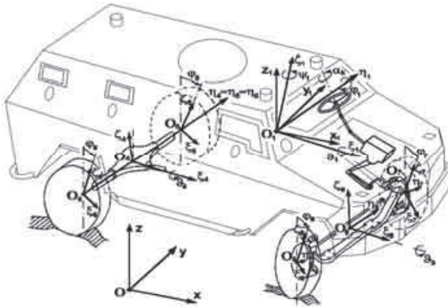
Fig. 2. A physical model of double axis light armoured vehicle and assumed coordinate systems [4]
