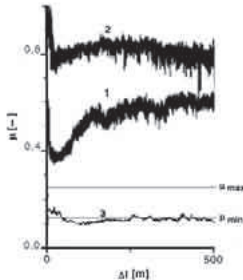
Fig. 10. Dry friction coefficient of a steel bearing-ball against Ti6Al4V \mu [14] vs. friction path \Delta l ; \mu_{\min} , \mu_{\max} – minimum and maximum calculated value for coefficient of friction obtained from measured maximum friction force T_{\max} between valve stem and its guide (Fig. 7; (a): 1 - substrate as delivered; 2 - diffusion hardened; 3 - nc-WC/a-C:H
