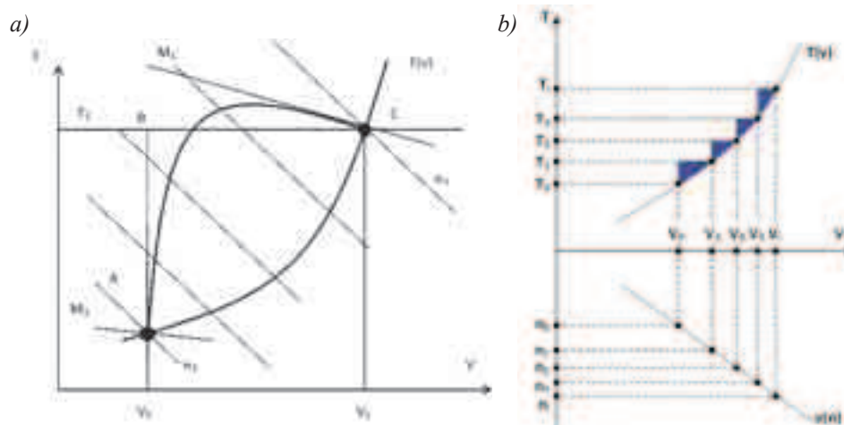
Fig.1. Models of rotational speed increase of the propeller in coordinates system: thrust (T) – ship's speed (v): a) successive increase of ship's speed; b) according to exploitation speed of the ship
