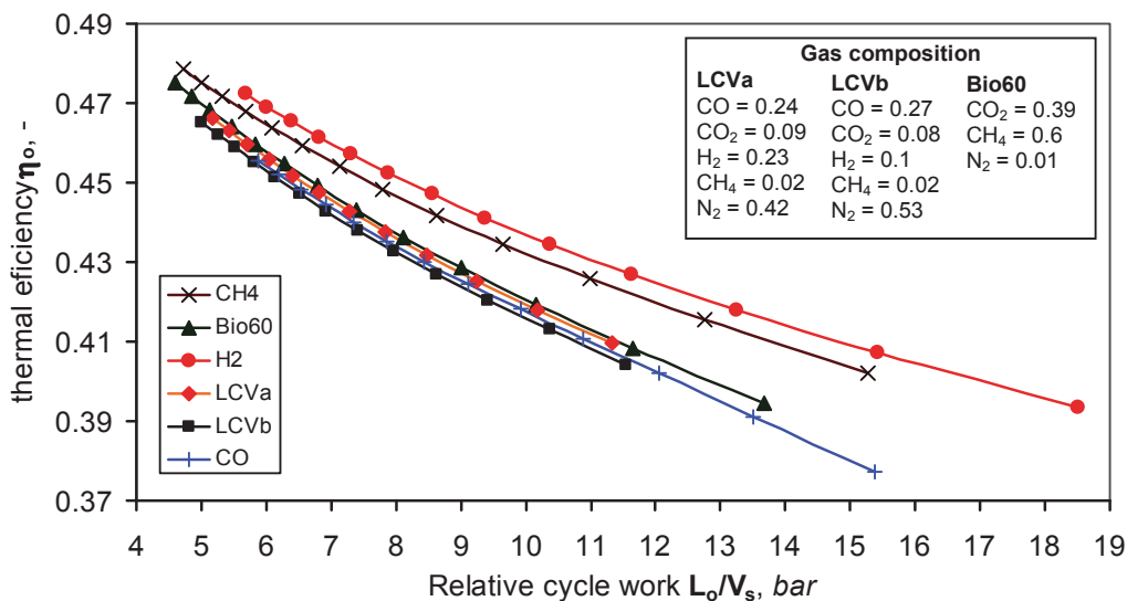
Fig. 5. The impact of relative cycle work L_0/V_s on the thermal efficiency of S-S cycle
