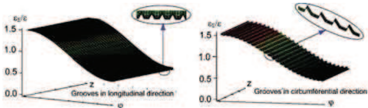
Fig. 2. The oil clearance in the crosswise slide bearing with micro-grooves
