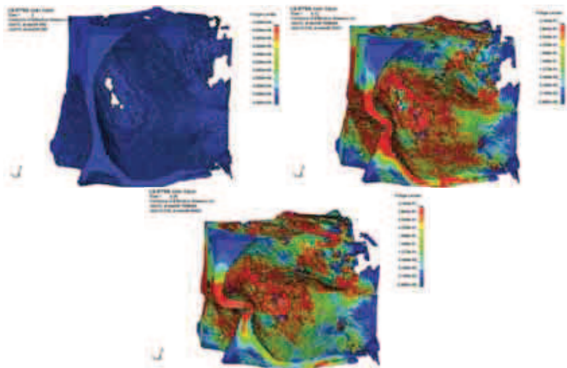
Fig. 7. Numerical analyses results as von Mises stress distributions for Sample 1
