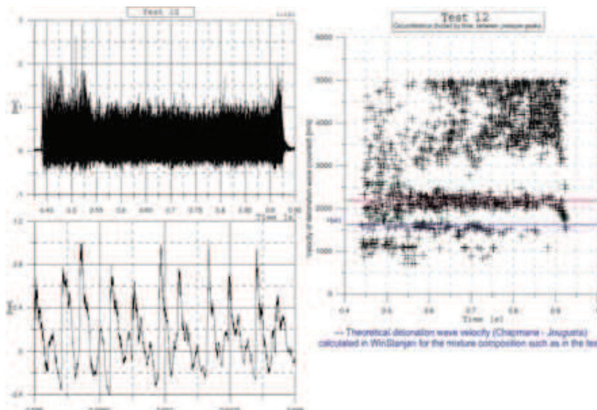
Fig. 4. Charts of pressure in the chamber and the calculated wave velocity
