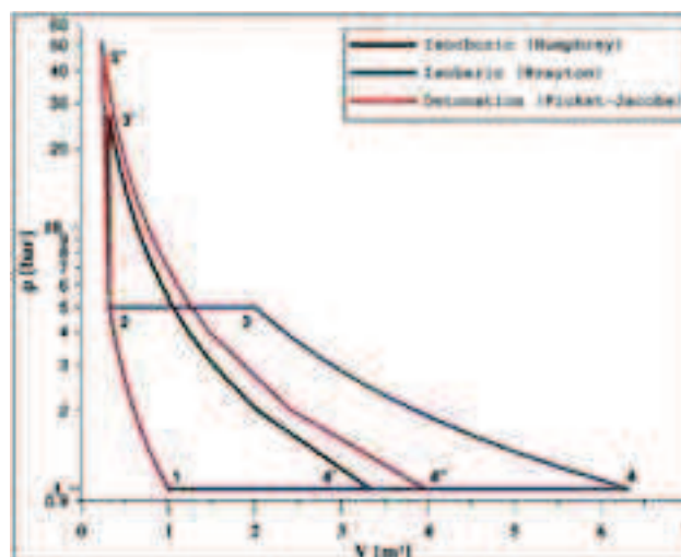
Fig. 1. Comparison of Humphrey and Brayton cycles with the theoretical detonation cycle (Ficket-Jacobs) [4]
