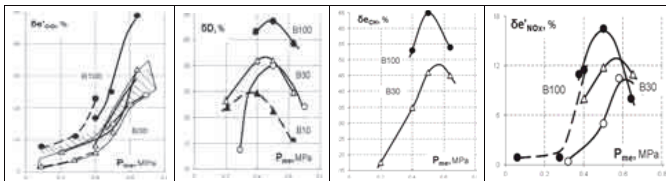
Fig. 1. The ecological parameters relative change of diesel engines F2L511 and 1A41 while running on biodiesel fuel: —●— B100 (F2L511, n=3000 rpm, unideal technical condition); —●— B100 (1A41, n=1750 rpm); —△— B30 (F2L511, n=3000 rpm, unideal technical condition); —○— B30 (F2L511, n=2000 rpm, unideal technical condition); — B30 (F2L511, n=3000 rpm, ideal technical condition); —△— B30 (1A41, n=1750 rpm); —▲— B10 (F2L511, n=3000 rpm, unideal technical condition)
