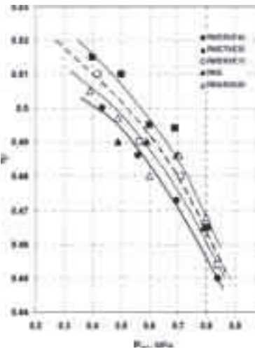
Fig. 10. Efficiency index of diesel engine 1A41
