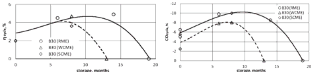
Fig. 21. Impact of the period of storage of B30 fuel on the overall efficiency factor
