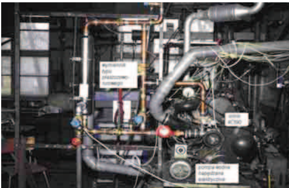
Fig. 2. Engine 4CT90 on the dynamometer with cooling system pressure
