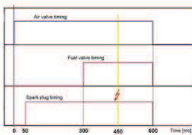
Fig. 5. Timing example of control gates that generate opening and closing signals to solenoid valves and firing signal to detonator
