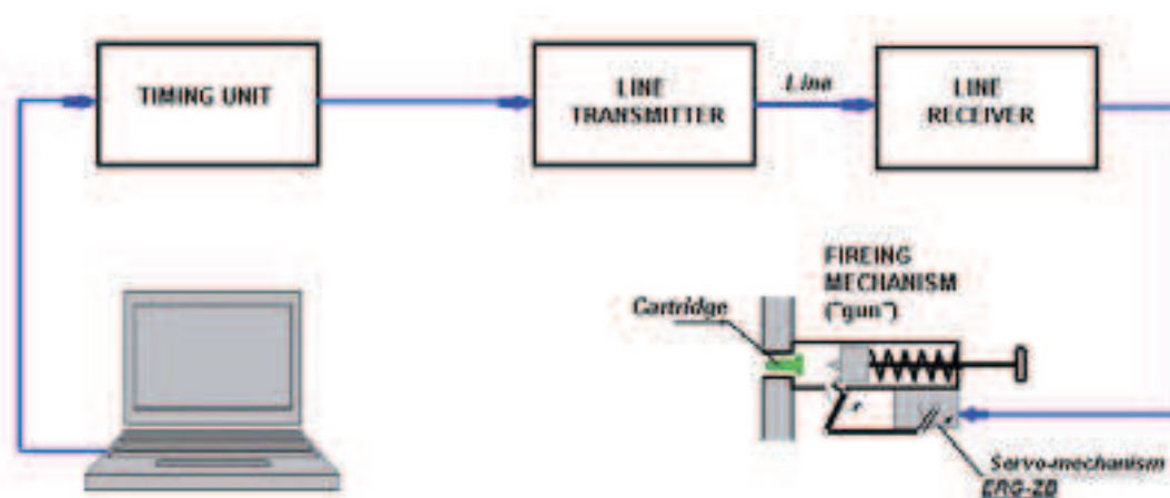
Fig. 7. Schematic diagram of system controlling of firing mechanism
