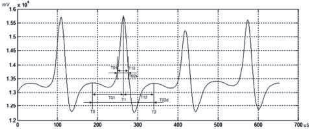
Fig. 3. Signal from the inductive sensor: T_{02d} , T_{02K} – respectively, long and short period of observation of a blade tip presence in the area of the sensor, T_0 , T_1 , T_2 – characteristic moments of observation of a blade tip under the sensor, T_{01} , T_{12} – sub-periods of observation of the blade tip respectively for T_d and T_k , mV – blade tip migration signal, \mu s – blade migration time
