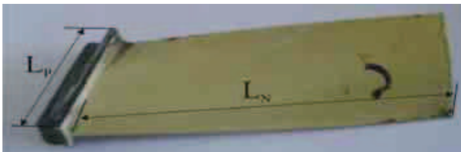
Fig. 1. I level compressor blades of the axial air turbine engine SO-3: L_N = 113 mm, L_P = 40 mm
