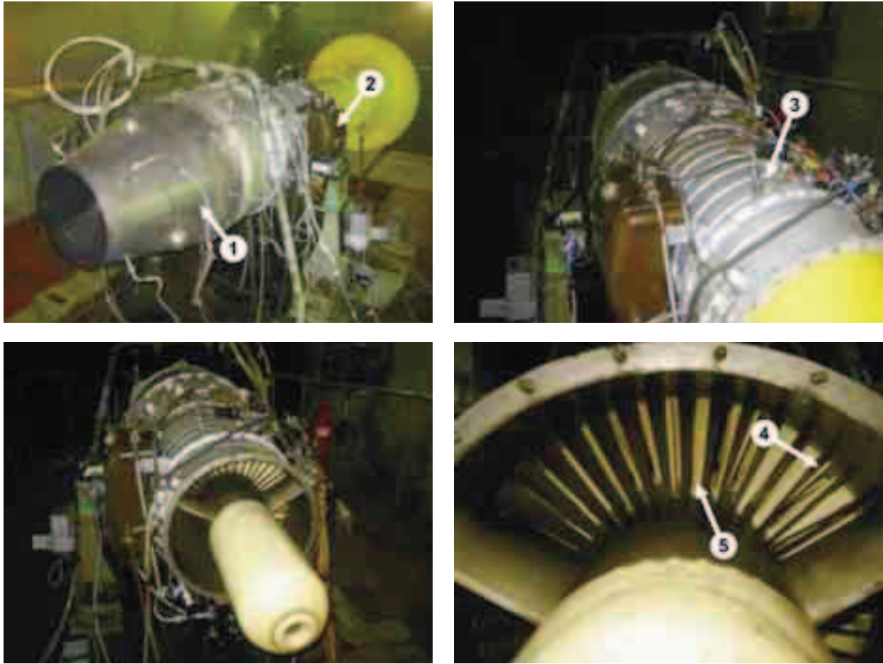
Fig. 2. Measuring station: 1 – turbine engine, 2 – measuring device, 3 – non-contact inductive sensor, 4 – compressor blades, 5 – guide blades
