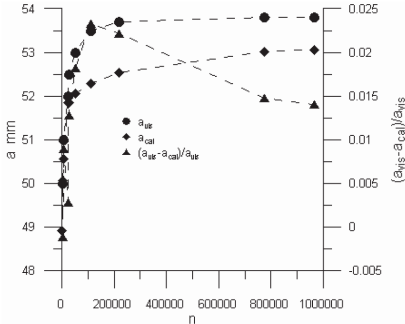
Fig. 3. Difference between the observed crack length a_{vis} and calculated crack length a_{cal} with the use of eq.1
