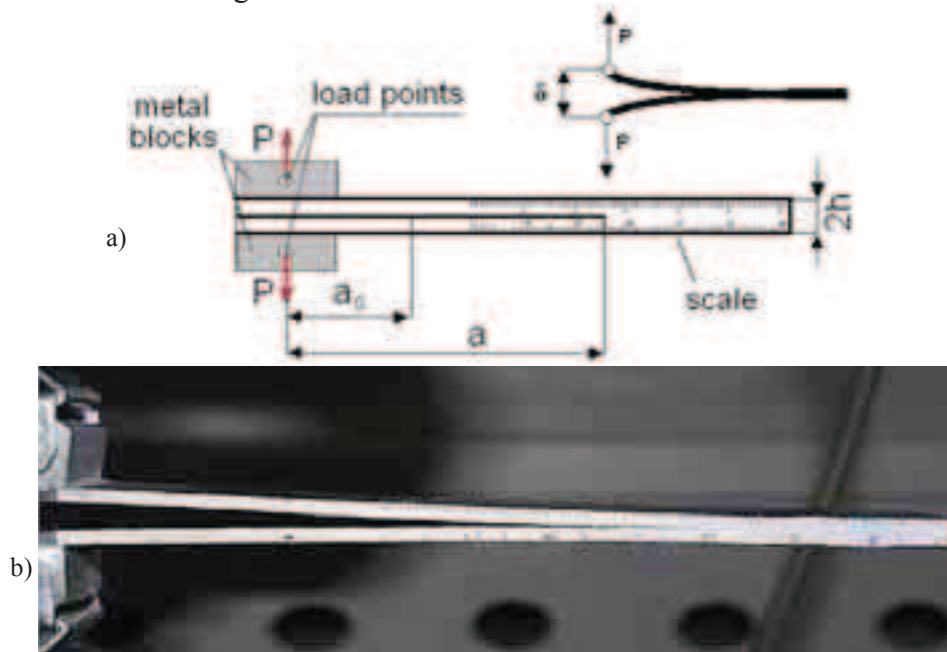
Fig.1. Double Cantilever Beam (DCB) specimens used for the determination of Paris-Erdogen law under Mode I cycling loading
