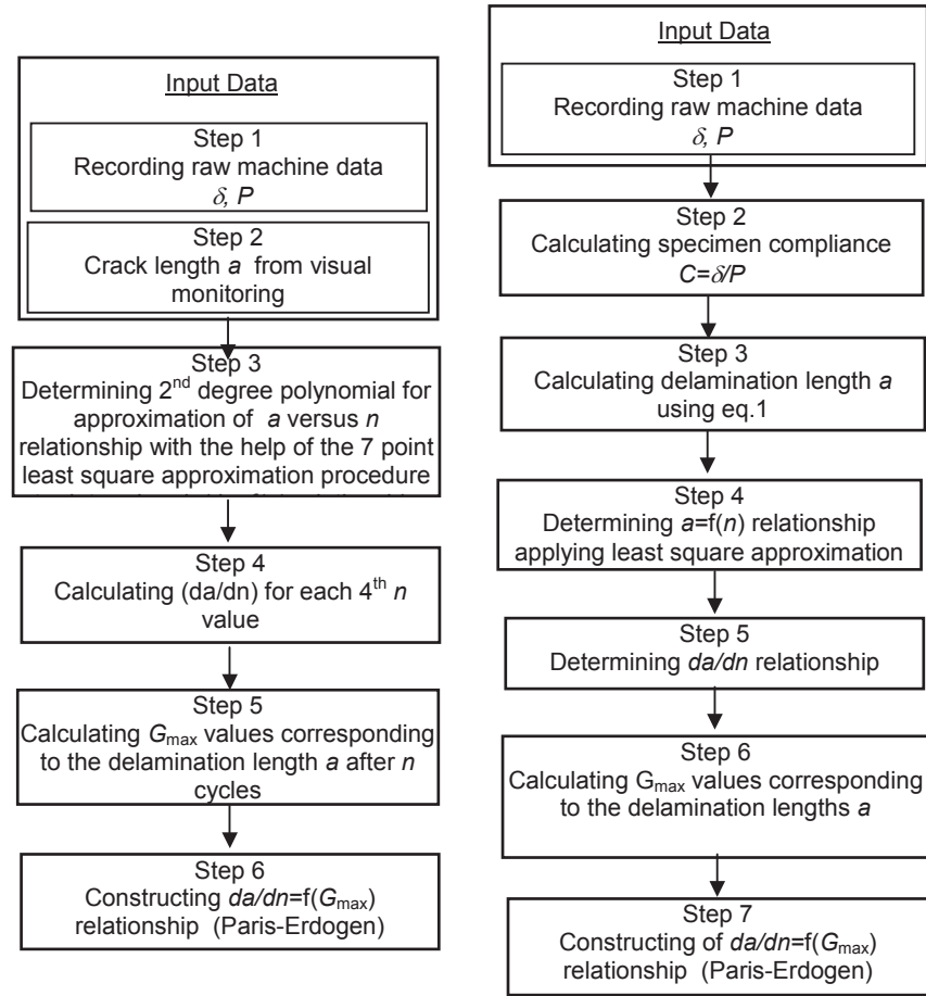
Fig. 1. ASTM E647 procedure, (left column) and proposed procedure (right column)
