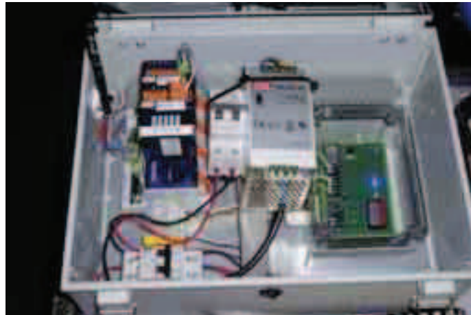
Fig. 3. Calculating module ETNP-10 with PLC SAI A
