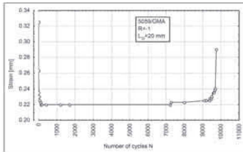
Fig. 3. Change of total strain amplitude \varepsilon_{ac} [mm] in dependence on the cycles number N obtained during the tests at \sigma_a = \text{const} (180.5 MPa). Initial total strain \varepsilon_c = 0.33 mm. ALUSTAR alloy welded with GMA (MIG) method (see Fig. 2)
