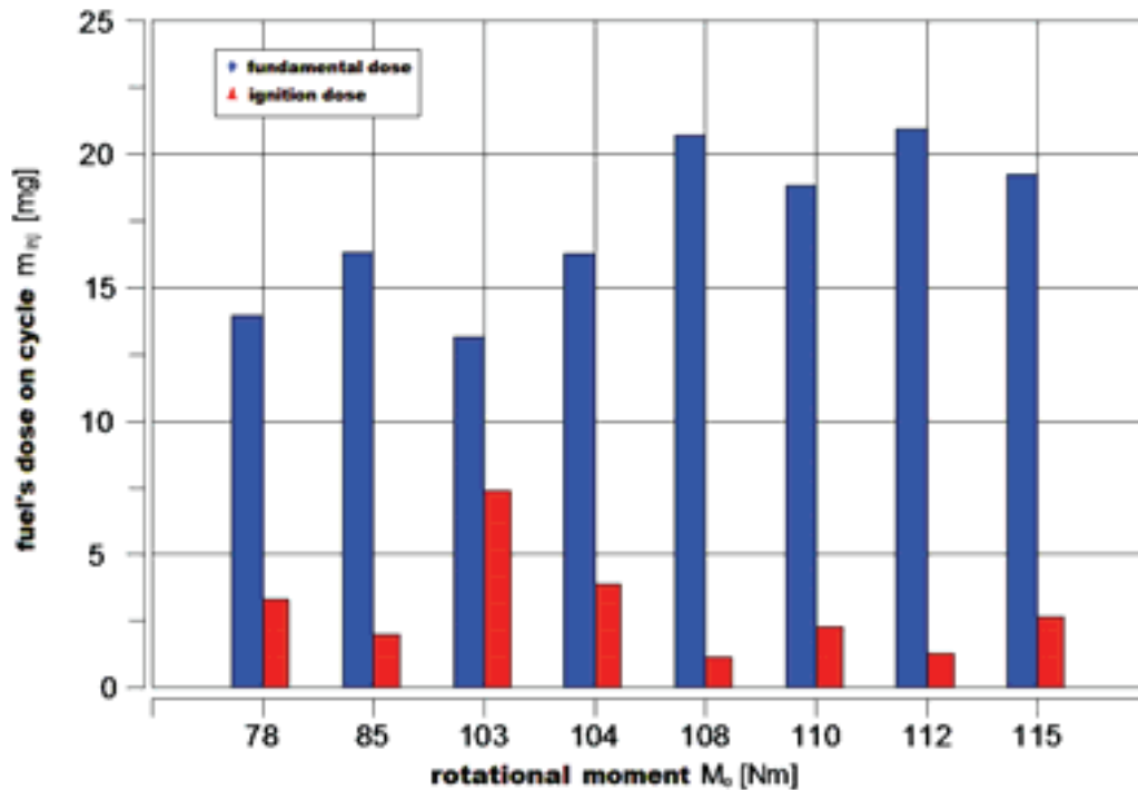
Fig. 4. Fuel doses size in the successive points of load characteristics of the engine working with the combustion initiation from the ignition dose at n = 2,000 [rpm]
