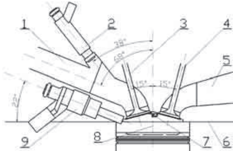
Fig. 2. Diagram of the location of the elements of the power supply systems for two-cycle engine 1 – approach duct, 2 – injection system of the fundamental dose (petrol), 3 – approach valve, 4 – escape valve, 5 – escape duct, 6 – surface of mutual location of head and block of engine, 7 – spark plug, 8 – axis of cylinder symmetry, 9 - ignition dose injection system
