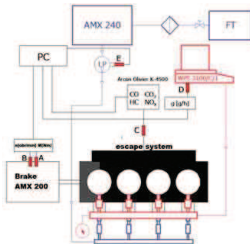
Fig. 1. Diagram of test bed (Symbols: A – measurement of rotational speed, B – measurement of rotational moment, C – measurement of coefficient of air surplus, and toxic components of the exhaust fumes, D – measurement of mass expense of the fuel, for the ignition dose injection, E – measurement of fuel consumption of fundamental dose)
