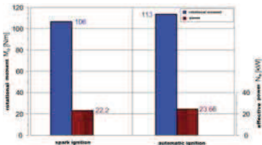
Fig. 5. Comparative diagram of the rotational moment and the effective power of the test engine working with the spark ignition and with the mixture combustion initiated from the ignition dose at n = 2000 [rpm]
