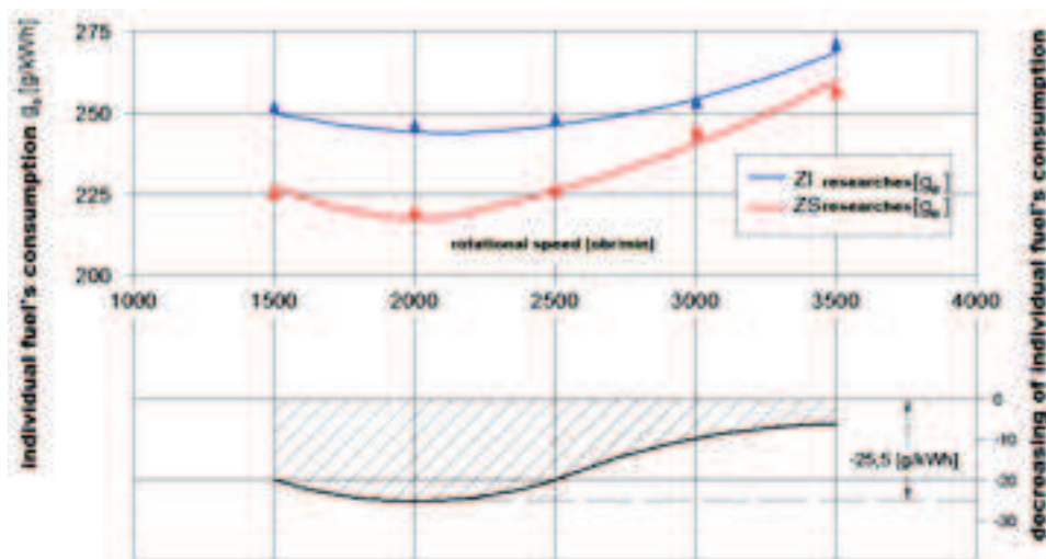
Fig.8. The course of the decrease of fuel consumption for the ignition dose, determined in relation to the work mode of a spark ignition, obtained based on test-stand research
