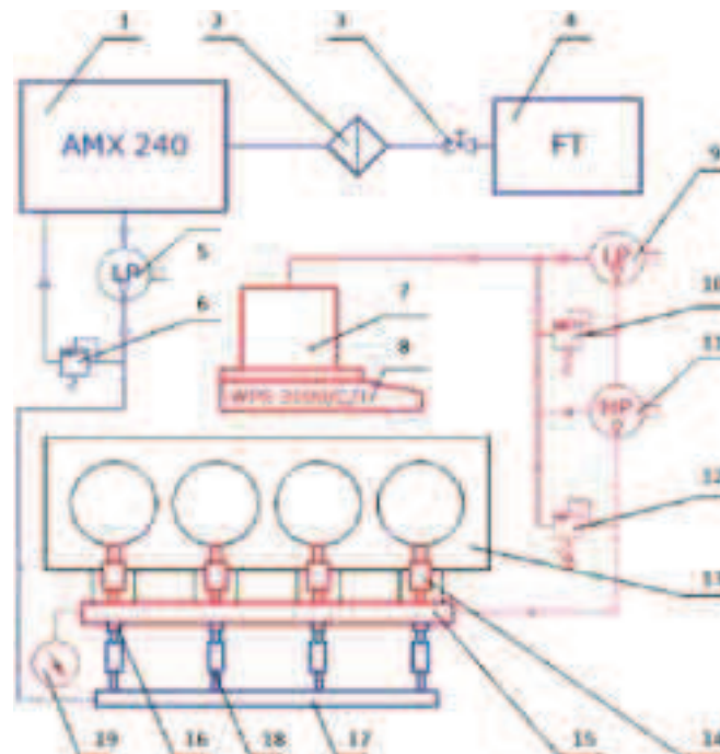
Fig. 3. Power supply system of the test engine (1– gravimetric fuels gauge, 2 – fuels filter, 3 – cutting off valve, 4 – fuels tank for MPI system, 5 – pump of fuel of petrol injection, 6 – controller of pressure of petrol injection, 7 – fuels tank for the ignition dose system, 8 – laboratory scales, 9 – powering pump system of ignition dose, 10 – controller of low pressure of circuit of ignition dose, 11 – pump of high pressure, 12 – pressure's controller of injection of ignition dose, 13 – test engine, 14 – ignition dose injection system, 15 – fuel rail of injection ignition dose systems, 16 – approach duct, 17 – fuel rail of MPI system, 18 – petrol injection system for MPI system, 19 – pressure manometer of the ignition dose injection)
