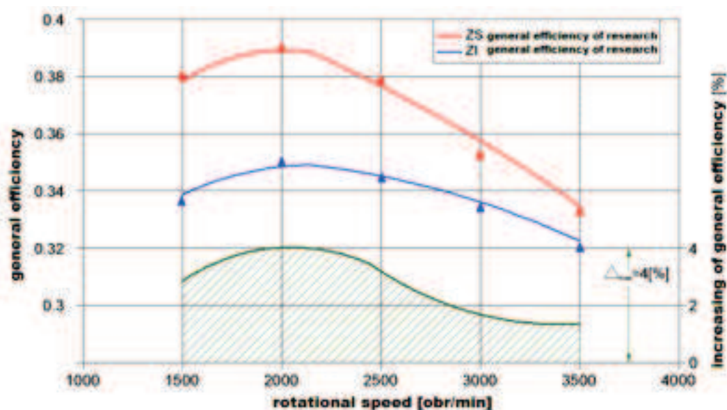
Fig. 9. The course of the increase of the general engine efficiency for the ignition dose determined in relation to the work mode of the spark ignition, set based on test-stand research
