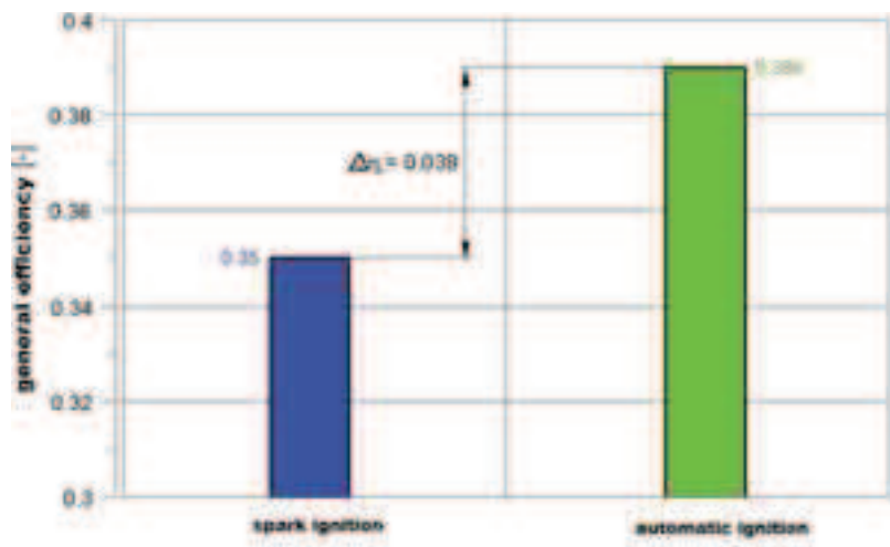
Fig.6. Comparison of general efficiency obtained by the engine working with the spark ignition and with the combustion initiated from ignition dose at n = 2000 [rpm]
