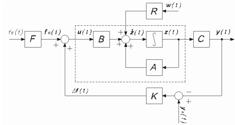
Fig. 2. Block diagram of an automatic control system with the input f_s(t)
