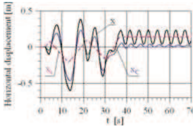
Fig. 6. Horizontal displacement
