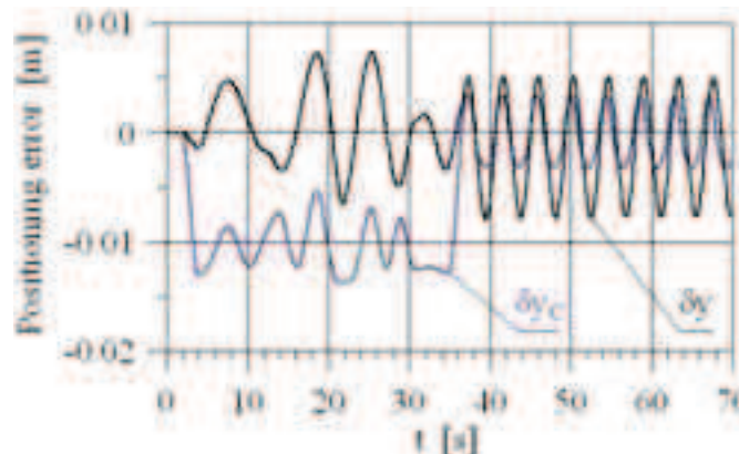
Fig 7. Positioning error
