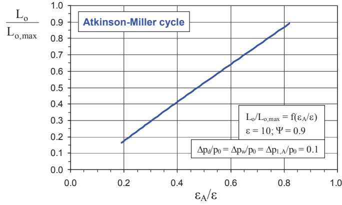
Fig. 7. Ratio of work of the open Atkinson-Miller cycle to the maximal work of the Seiliger-Sabathe cycle versus control parameter \varepsilon_A/\varepsilon
