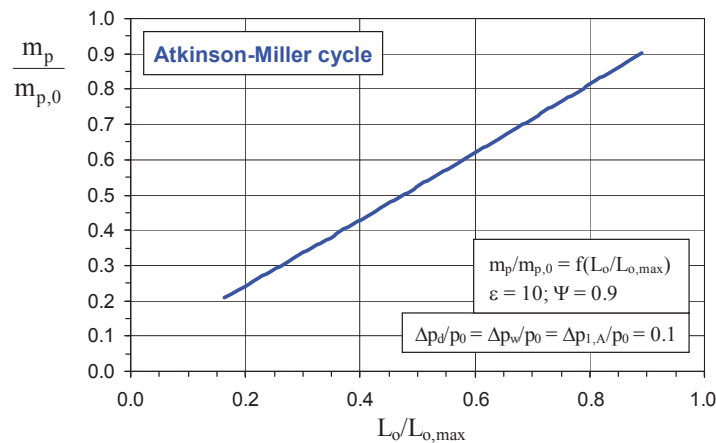
Fig. 4. Relative fuel dose m_p/m_{p,0} versus work of the open Atkinson-Miller cycle
