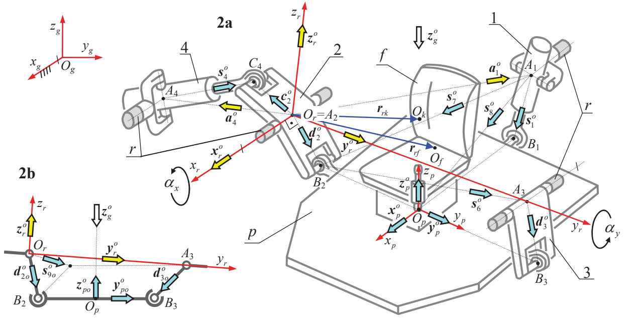
Fig. 2a, b. Vectors and versors in the kinematic model of cab suspensions
