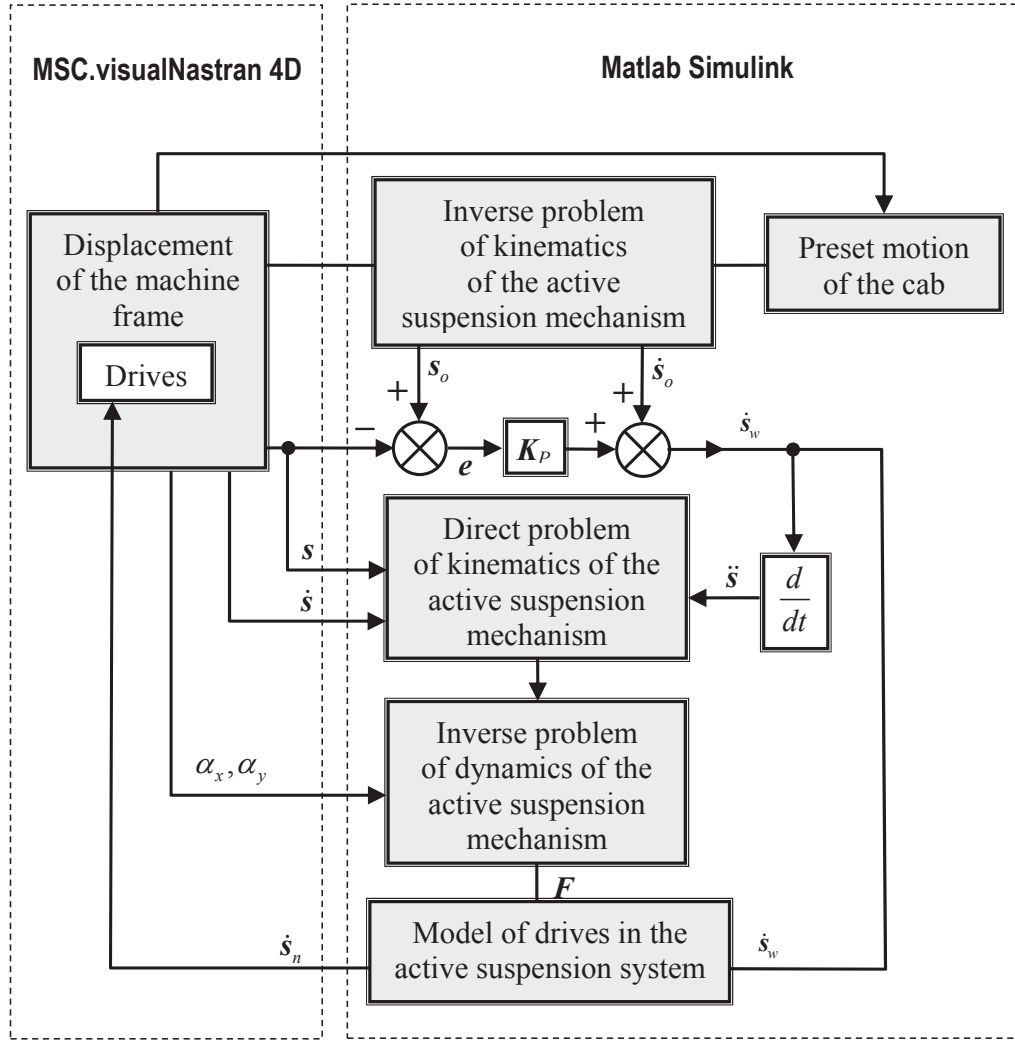
Fig. 4. Model of drives control in the active suspension system - schematic diagram
