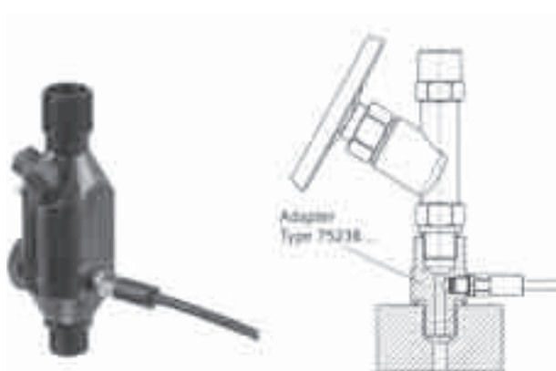
Fig. 4. Sensor's connecting adapter before the indicator cock
