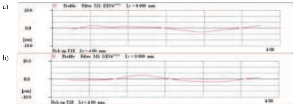
Fig. 2. Examples of waviness profiles of Ni-Al coatings obtained by plasma spraying: a) the turned ( W_t = 3.47 \mu m ), b) the burnished ( W_t = 3.6 \mu m )
