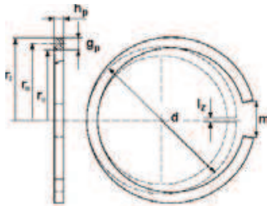
Fig. 3. Sketch of the compression ring
