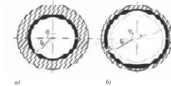
Fig. 5. Sketch of ring installed in new (a) and worn (b) cylinder
