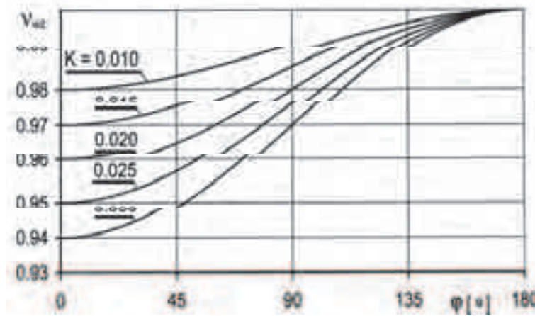
Fig. 4. Ring relative curvature variations draft for selected values of K parameter
