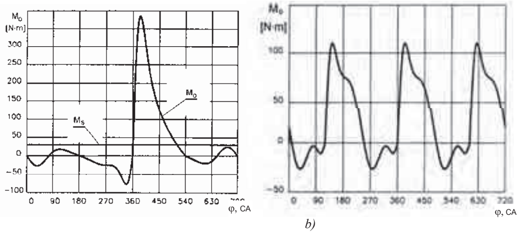
Fig. 1. Exemplary torque courses of one-cylinder (a) and three-cylinder (b) 4-stroke engines; M_s – mean torque [3]
