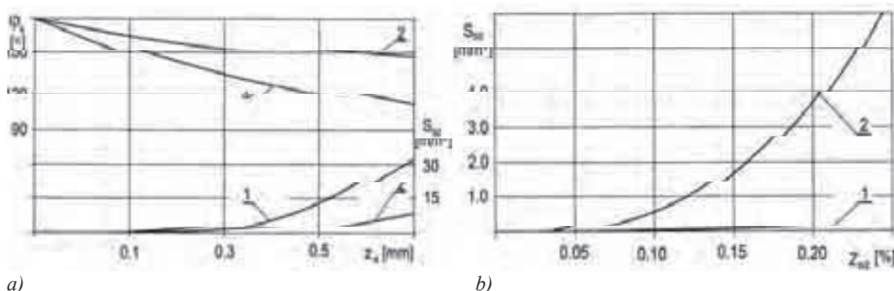
Fig. 6. Variations in \varphi_k angle and area of S_{sz} slot vs. absolute z_a and relative z_{wz} value of cylinder wear for an automotive (1) and marine (2) engine
