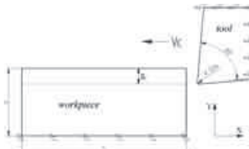
Fig. 2. Boundary conditions
