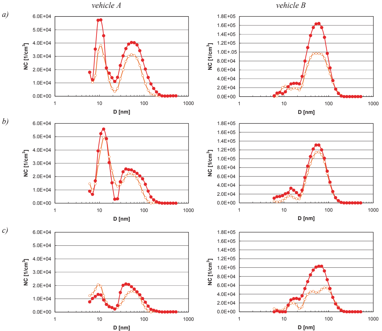
Fig. 8. Normalized particle number NC as a function of diameter D recorded on different road portions for vehicles A and B: a) urban, b) extra urban, c) expressway; ● – drive with load, ○ – drive without load
