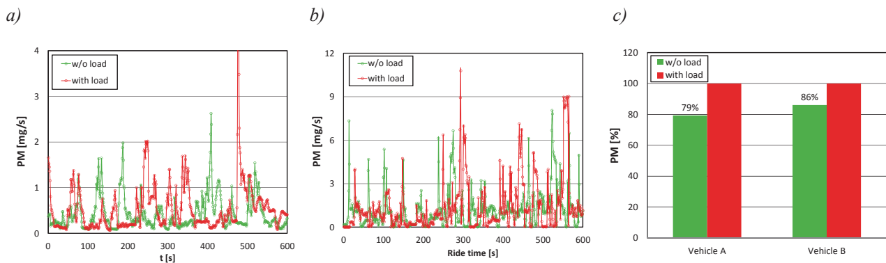
Fig. 4. PM emission rate on the urban road portion: a) vehicle A, b) vehicle B, c) relative values
