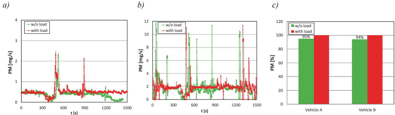
Fig. 6. PM emission rate on the expressway road portion: a) vehicle A, b) vehicle B, c) relative values
