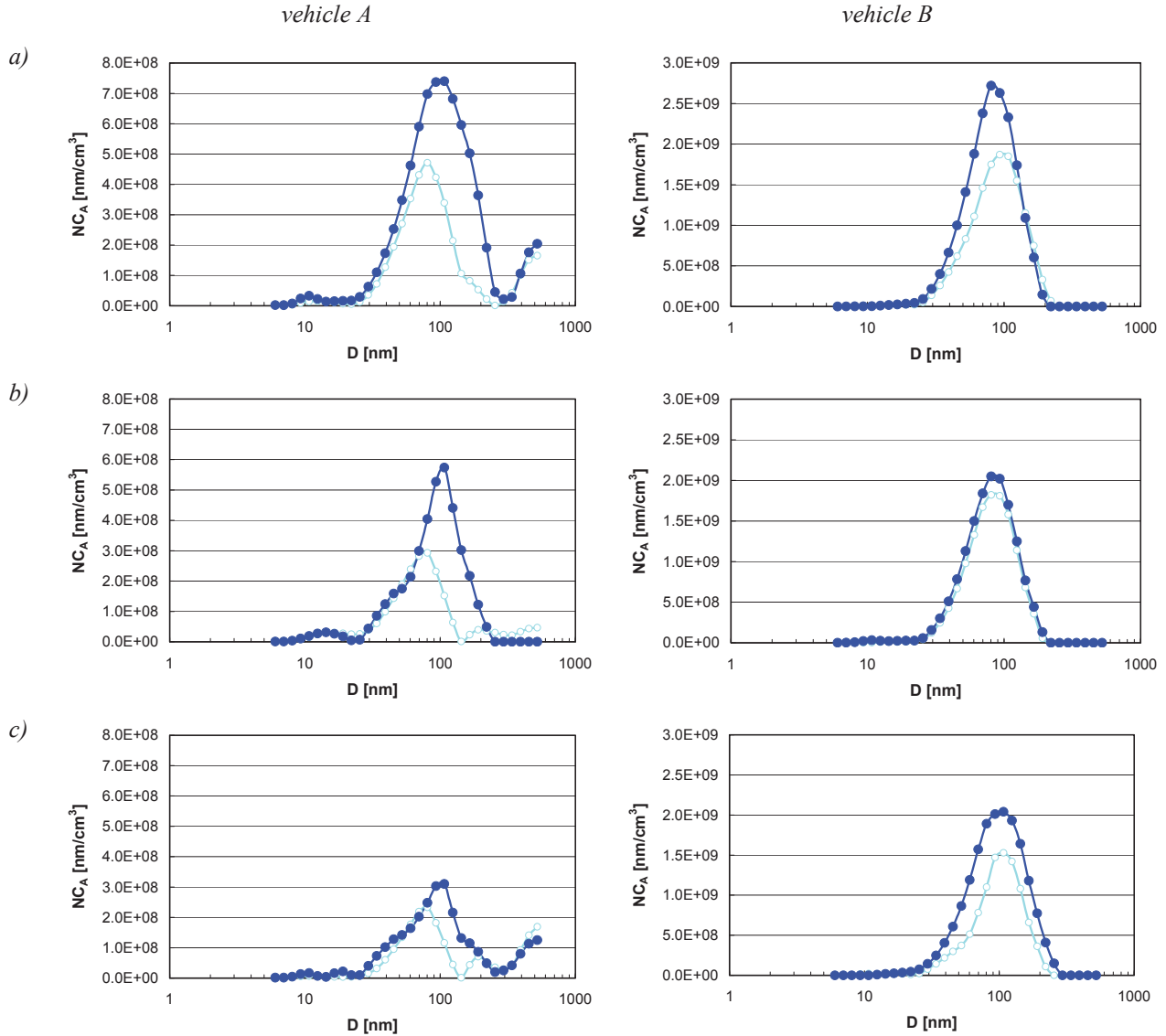
Fig. 9. Normalized surface concentration NC_A of PM as a function of diameter D recorded on different road portions for the tested vehicles A and B: a) urban, b) extra urban, c) expressway; ● – drive with load, ○ – drive without load
