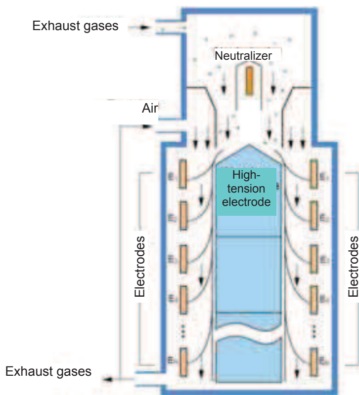
Fig. 2. Schematics of the EEPS 3090 particle sizer
