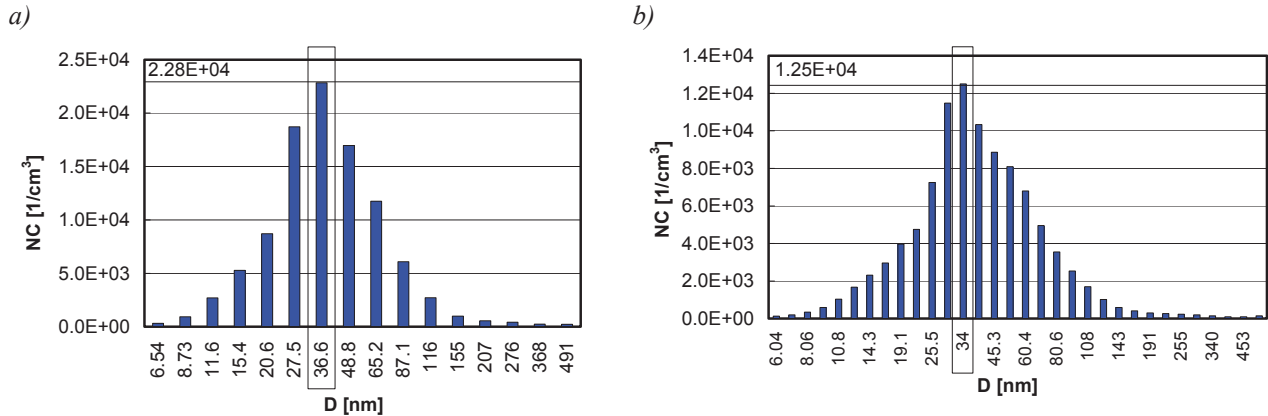
Fig. 7. Comparison of the normalized particle number depending on the diameter D using: a) 16 measurement channel analyzer, b) 32 measurement channel analyzer
