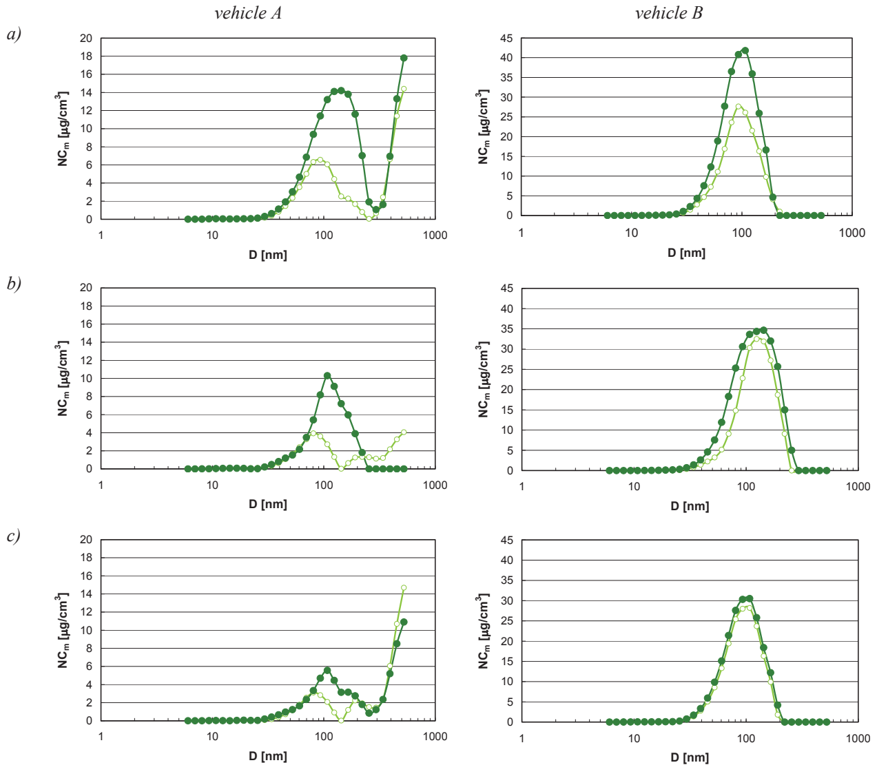
Fig. 10. Normalized mass concentration of PM NC_m as a function of its diameter D recorded on different road portions for vehicles A and B: a) urban, b) extra urban, c) expressway; ● – drive with load, ○ – drive without load
