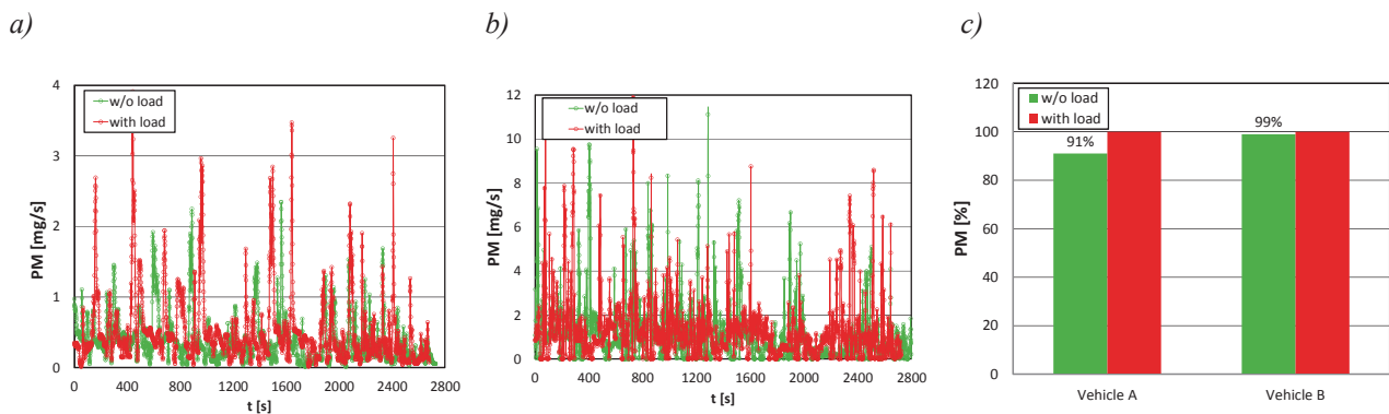
Fig. 5. PM emission rate on the extra urban road portion: a) vehicle A, b) vehicle B, c) relative values
