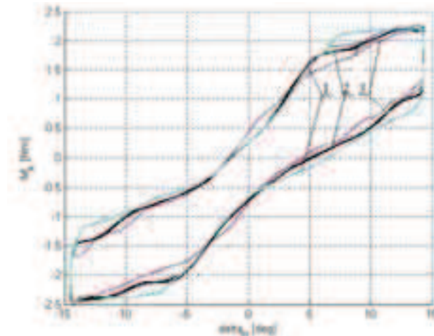
Fig. 12. Plot of steering wheel torque versus steering wheel angle at different input function frequencies. Vehicle speed 0 km/h; frequencies: 1 – 0.5 Hz, 2 – 1.0 Hz, 3 – 1.5 Hz
