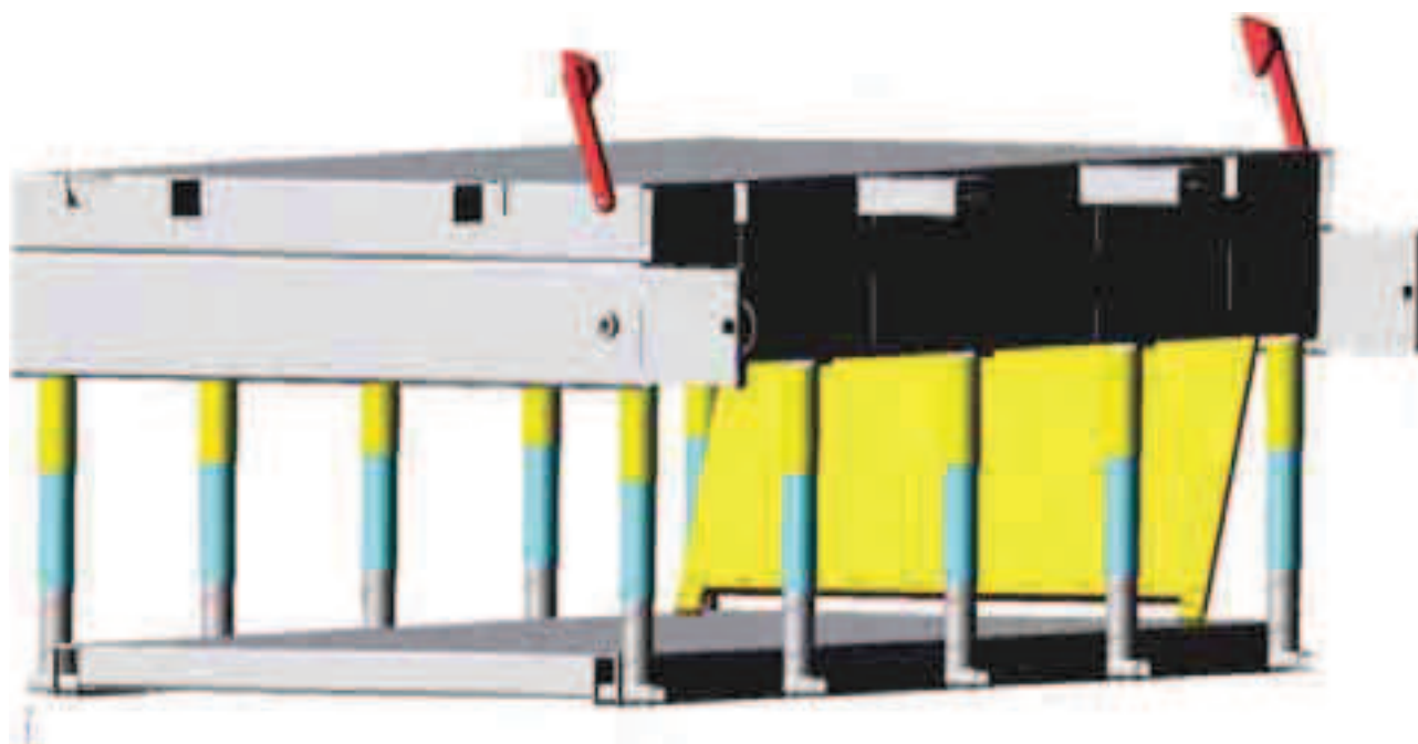
Fig. 2. 3D model of floating cassette with visible subsystems of mechanism of lowering the bottom and elements of movable lock (without elastic pontoon)
