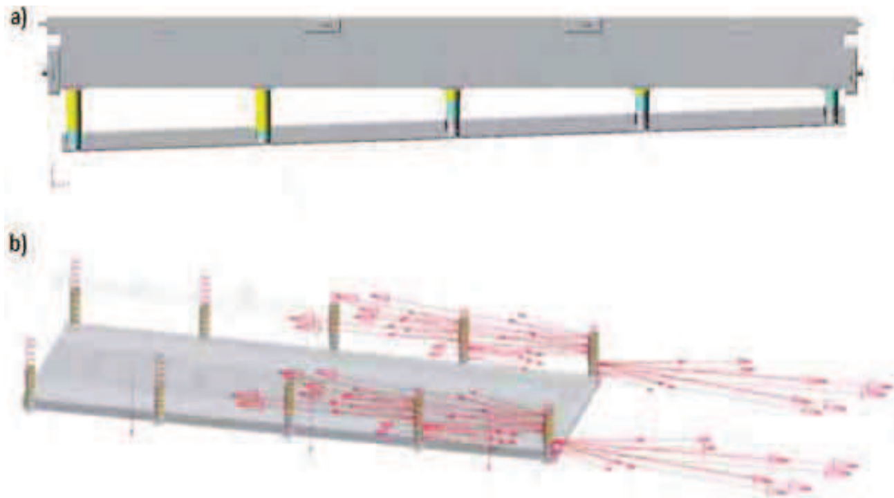
Fig. 5. Distribution of vectors of contact forces between telescopic mechanisms cylinder corresponding to the state of seizing and incomplete displacement of the bottom – variant I of the simulation
