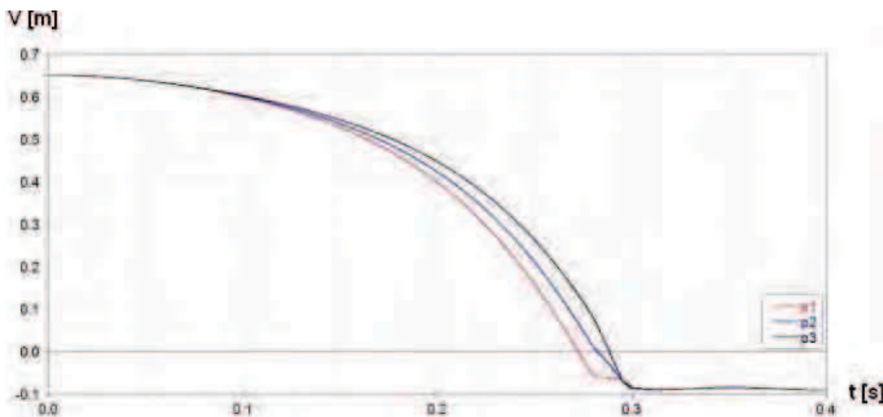
Fig. 6. Displacement of measurement points P_1 , P_2 and P_3 on the cassette bottom – variant III
