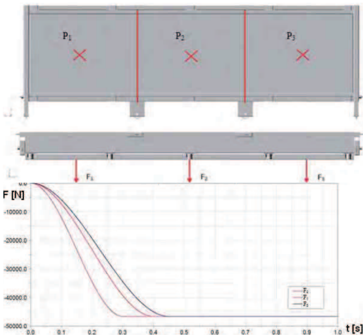
Fig. 4. Distribution of points of measuring displacements on the bottom of the cassette and reduced loadings F from pressure of the elastic pontoon filled with the air in time 1s – variant I
