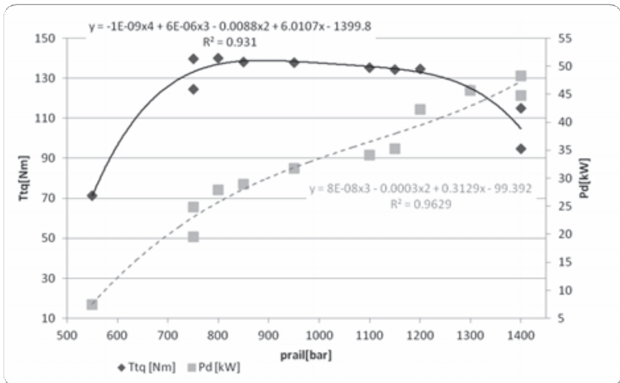
Fig. 5. Torque and engine power output to CR pressure relationship
