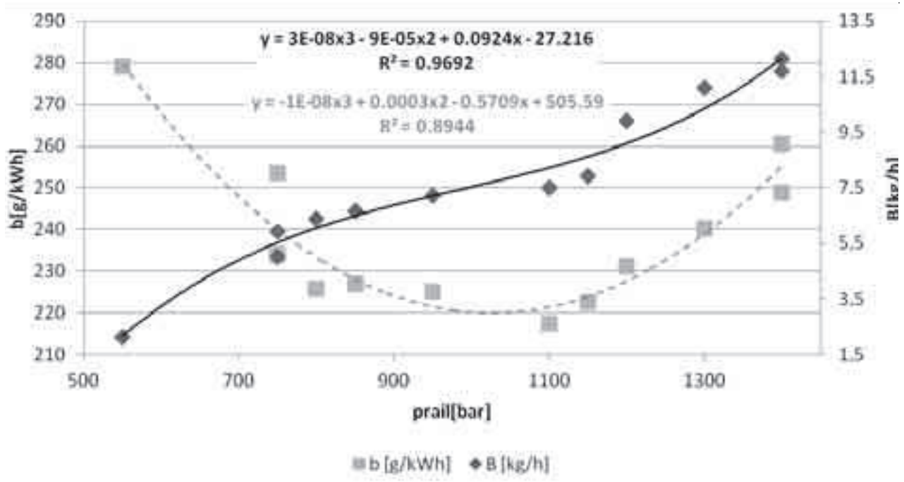
Fig. 6. Specific and hourly fuel consumption to CR pressure relationship
