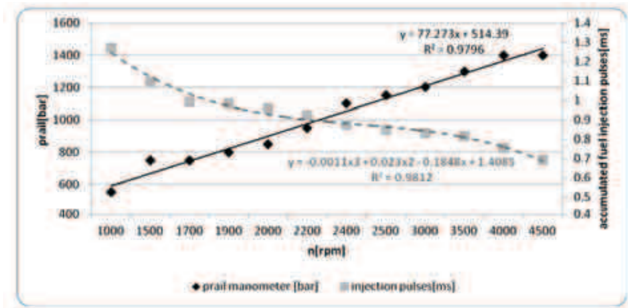
Fig. 4. CR pressure and accumulated fuel injection pulse to engine speed relationship
