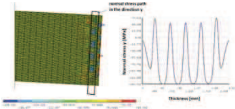
Fig. 13. Normal stresses \sigma_y in cross-section of preloaded material in plastic range of metal component next loaded by bended moment
