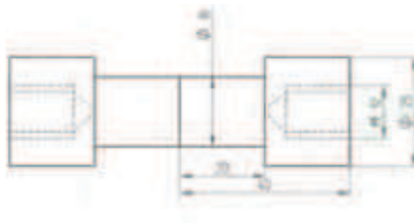
Fig. 2. Shape and dimensions of butt specimens
