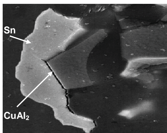
Fig. 6. Fractures on the boundary of the intermetallic compound grain CuAl 2 in AlSn20 alloy [4]
