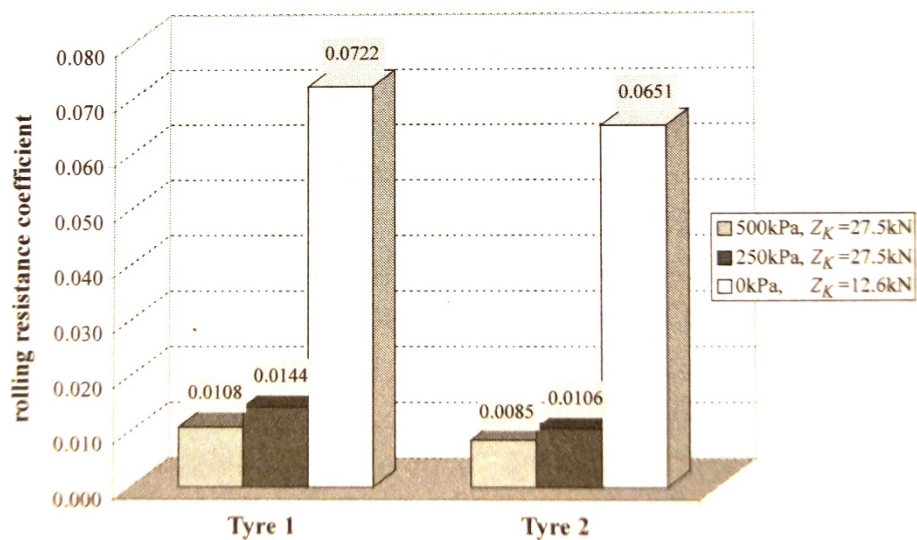
Fig. 9. Rolling resistance specification for two types of RFT tires 14.00R20, applied in a military vehicle [1]
