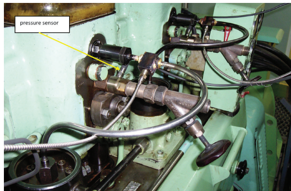
Fig. 1. Pressure sensor Kistler installed in indicator cock
